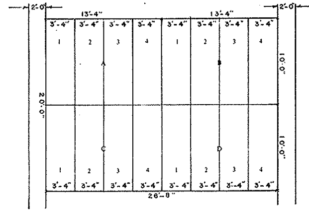
Typical Plot Plan Scale 1"=5'-0"
