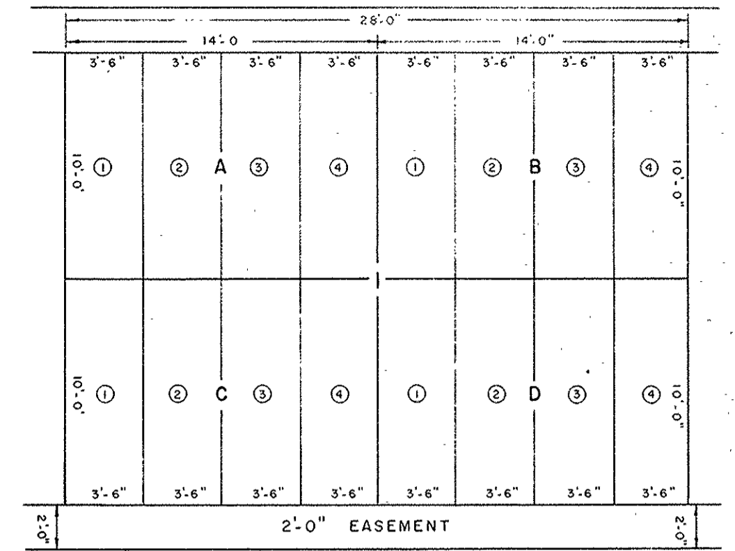
TYPICAL PLOT PLAN (SCALE: 1"=6'-0")
