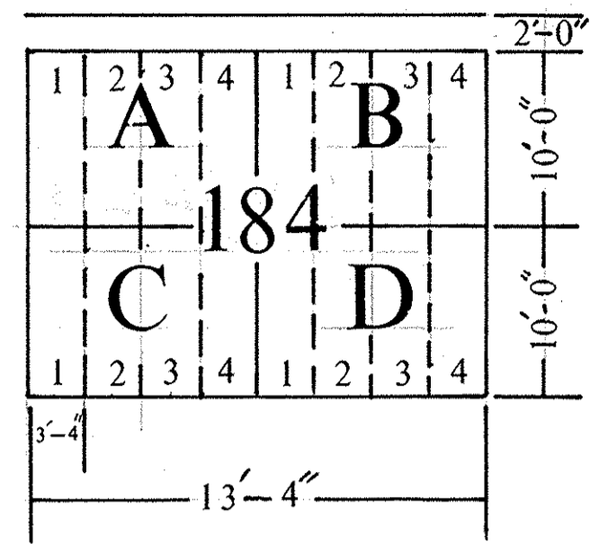
TYPICAL PLOT LAYOUT scale: 1"=10'
