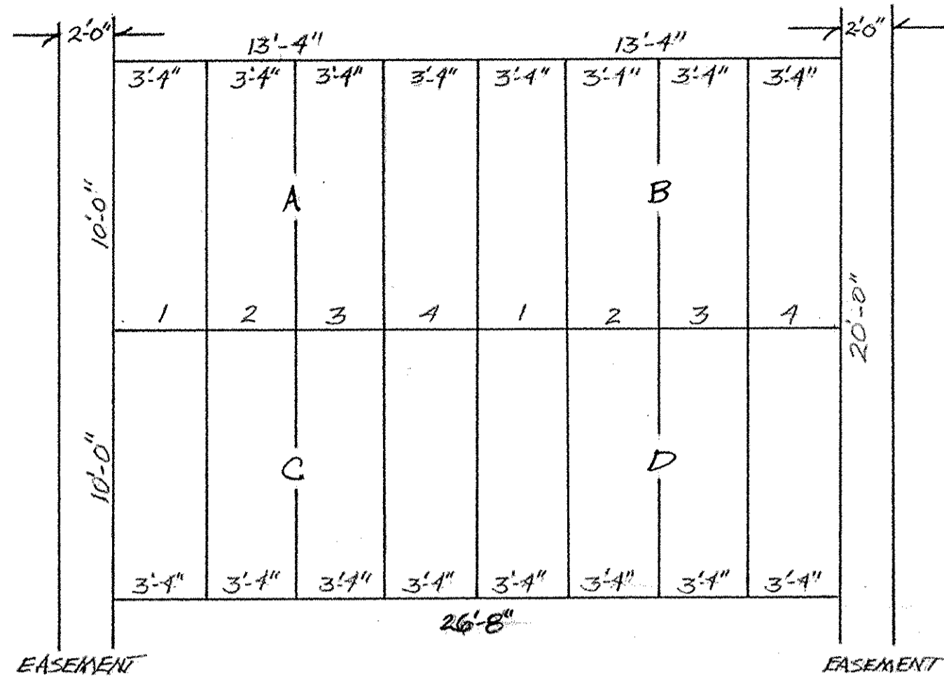
TYPICAL PLOT LAYOUT SCALE: 1" = 5'-0"
